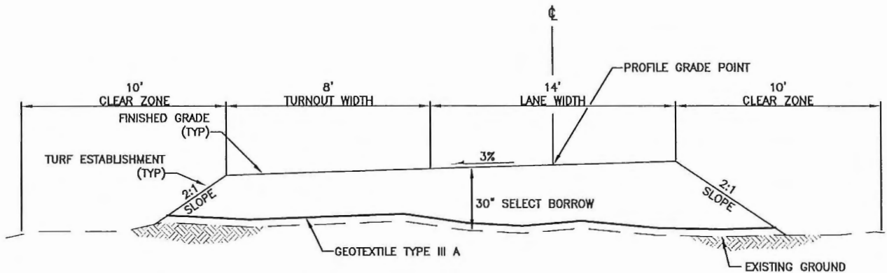
B ONE-LANE TWO-WAY ROAD TURNOUT SCALE: NTS
