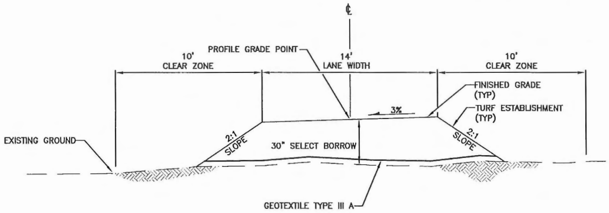
A ONE-LANE TWO-WAY ROAD SECTION SCALE: NTS
