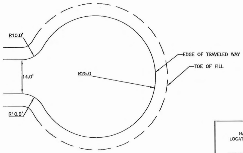
C TURN AROUND SCALE: NTS
